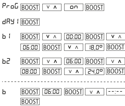
Fig. 3: Programming example
