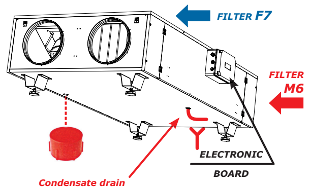
TYPICAL OPERATION
