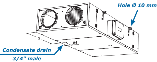
ENY-P1-S / ENY-P2-S / ENY-P3-S
