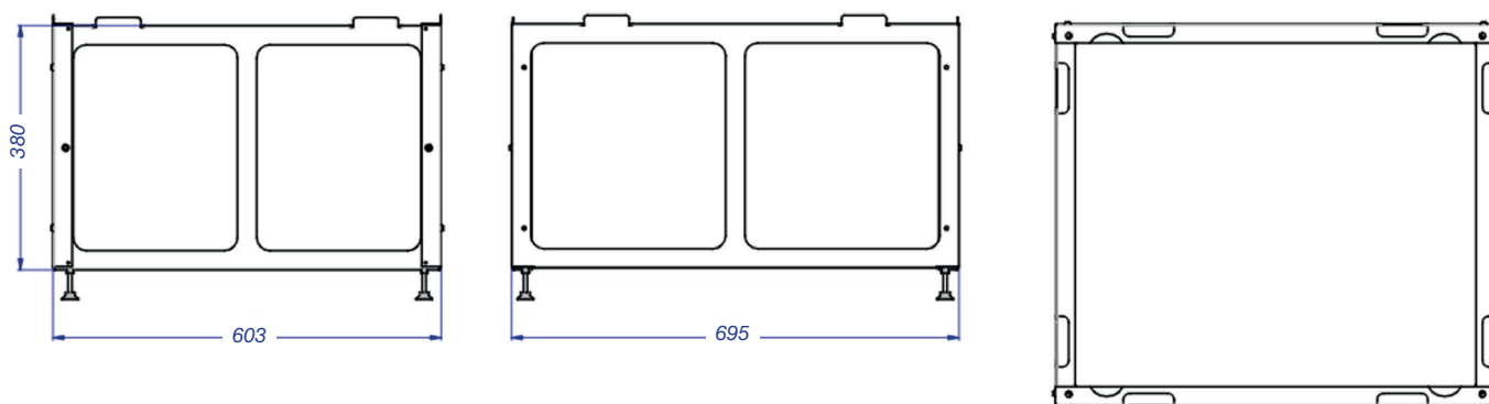
Support de montage DX (E) Horizontal
