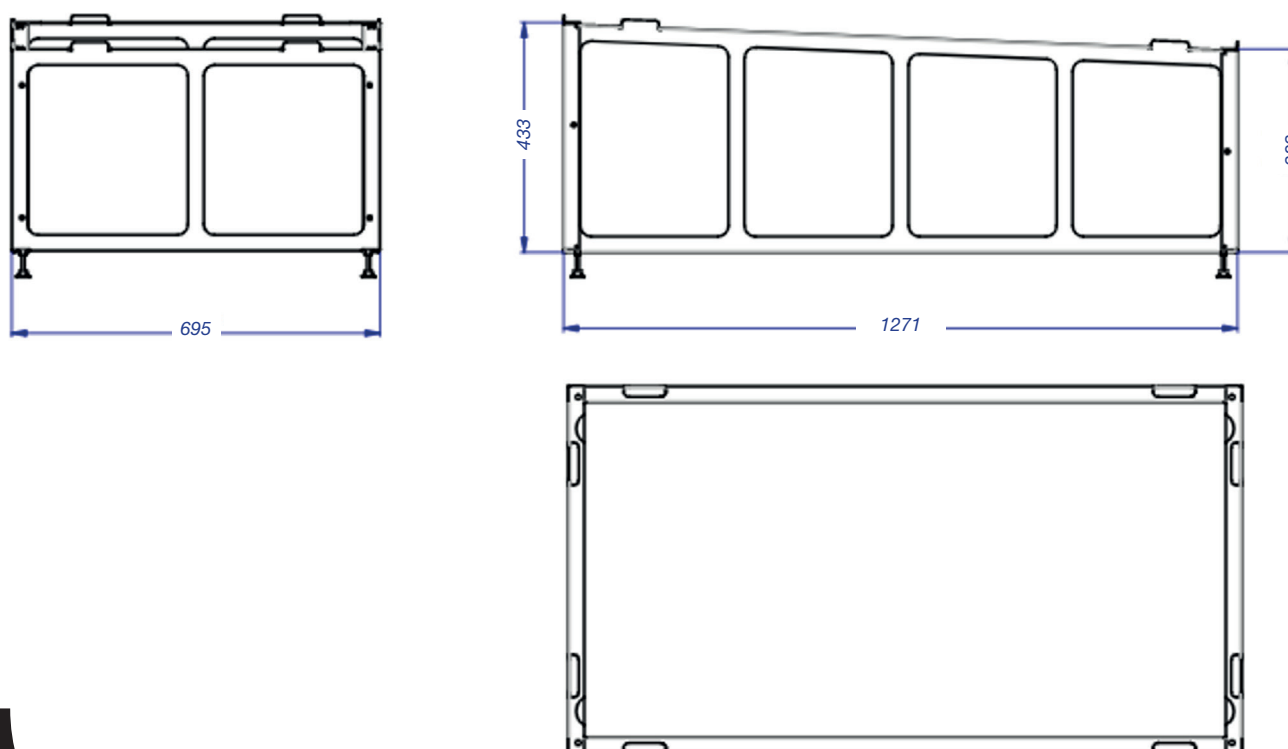
Support de montage DX (E) Horizontal
