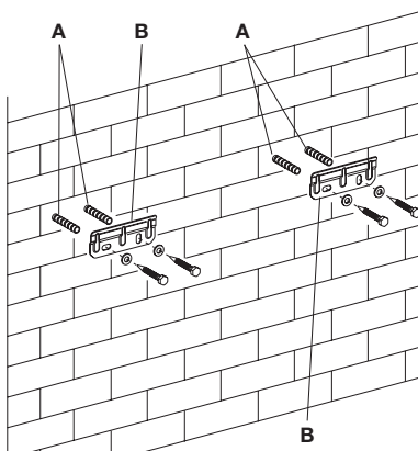
brackets
