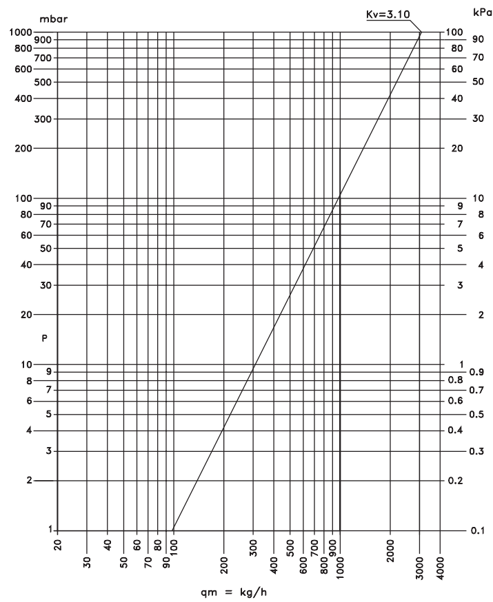
diagram of load losses of 3-way valve, in completely closed position.
