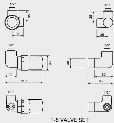
1-8 VALVE SET
