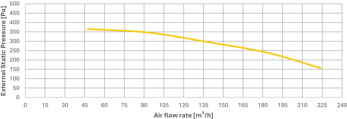
Characteristic curve
