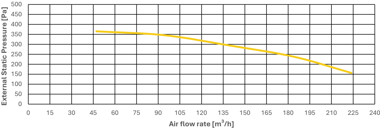
Characteristic curve
