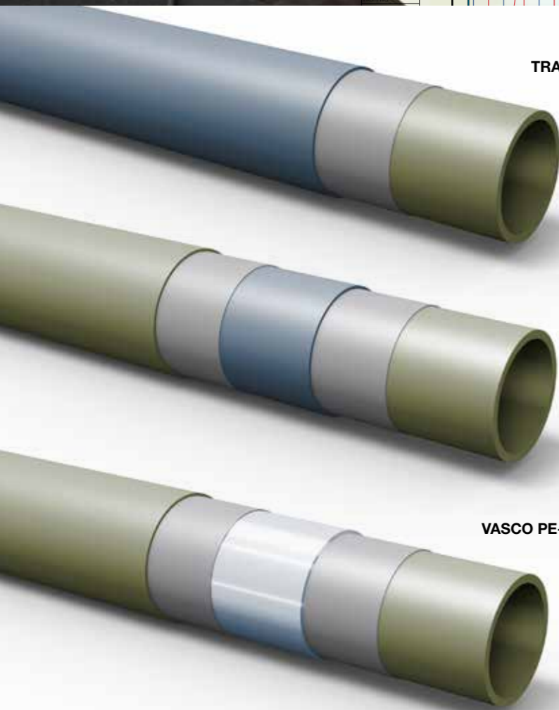
VASCO PE-XA (5 layer pipe)
