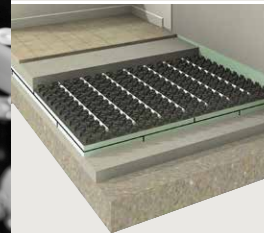
Wet Knob System
