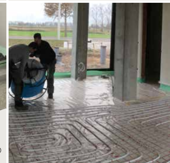
Wet Knob System
