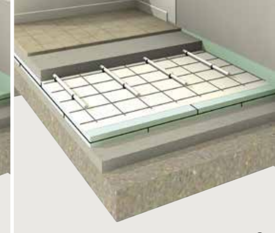
Wet Grid System
