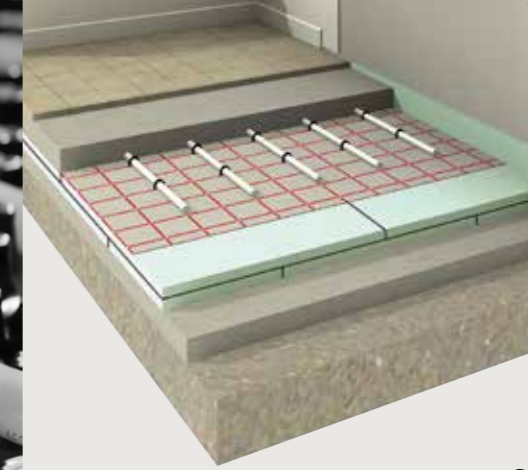
Wet Tacker System
